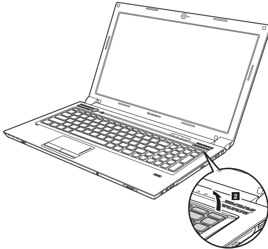
Figure 8. Removal steps of keyboard (continued)
